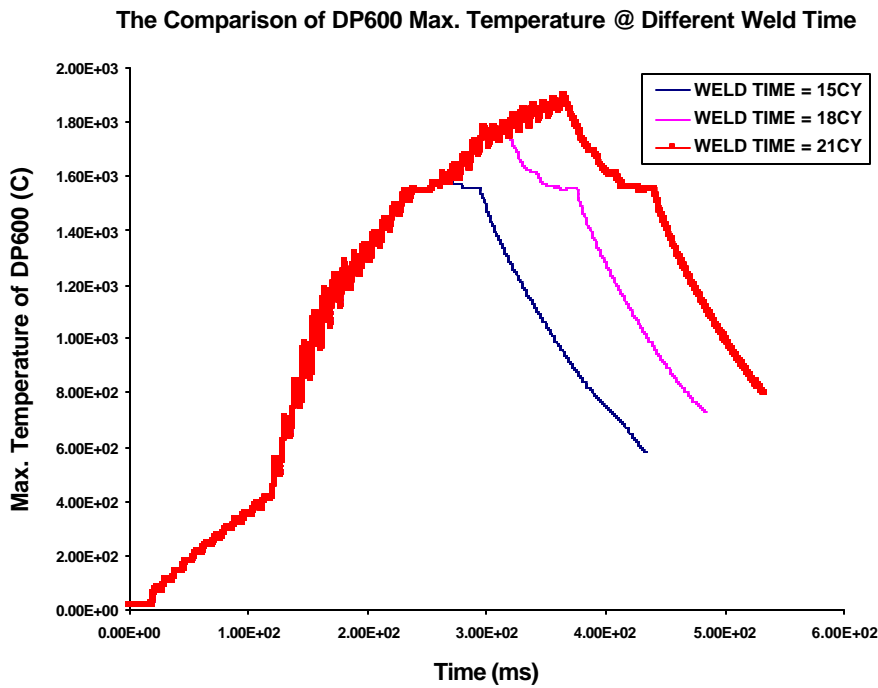
Figure 3. Maximum temperature of one-pulse welding with different weld times simulated by SORPAS software.
