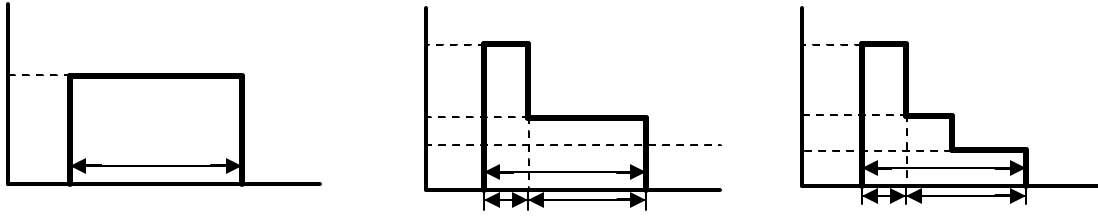
Figure 2. Types of current inputs tested; from left to right, a single pulse weld, a two-pulse weld and a three-pulse weld.
