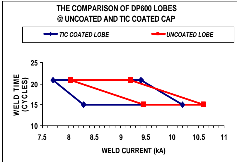
Figure 10. Experimental results illustrating welding lobe of coated and uncoated electrodes of single-pulse welding time.
