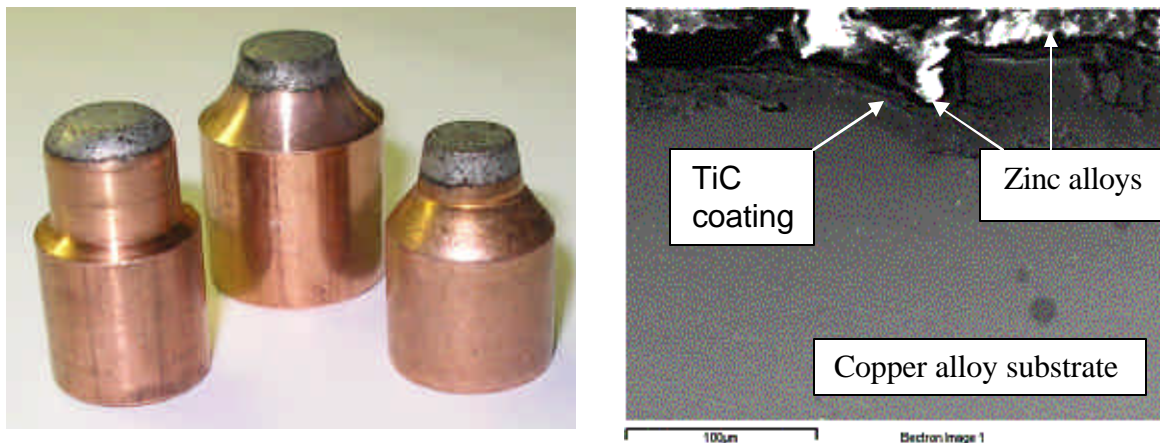
Figure 5. Left are titanium carbide-coated electrodes (TiCap) and, right, an SEM cross-section of a used TiCap showing the coating's effectiveness in retarding molten zinc alloys' attempt to migrate, once vapourized in welding, into the copper alloy electrode.
