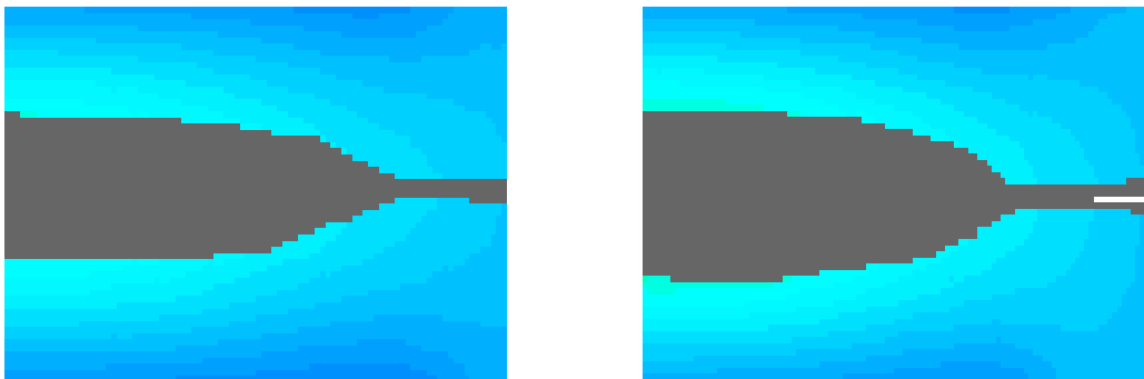
Figure 1. Nuggets simulated by SORPAS software, using a two-pulse current; on the left is a two-cycle first pulse, on the right a five-cycle first pulse.
