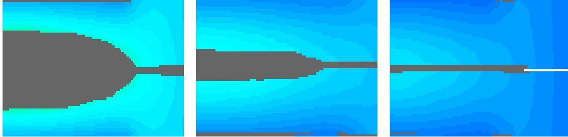
Figure 4. SORPAS software generated nugget profiles at 4, 5 and 6 kN, respectively.
